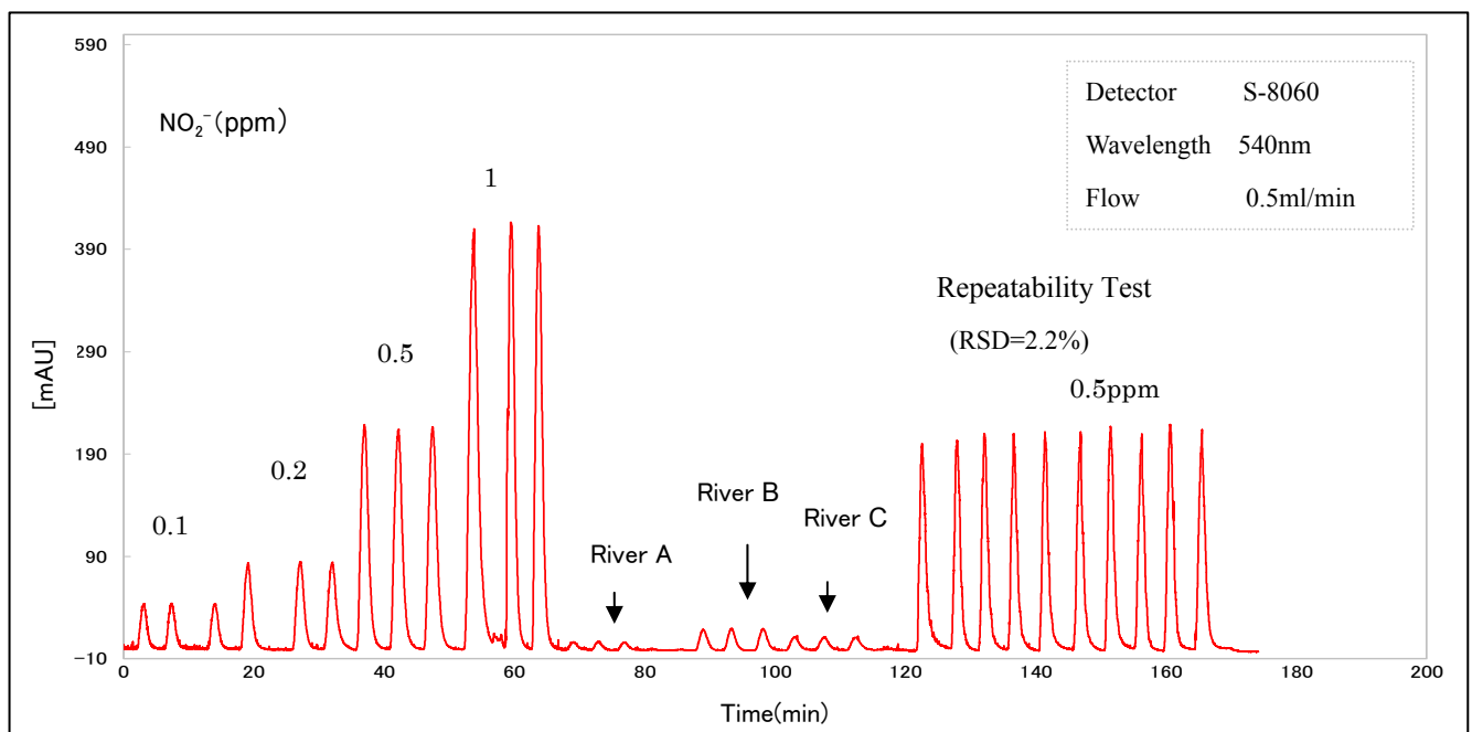
Flow signal of standard solution and river water, (Repeatability Test)
